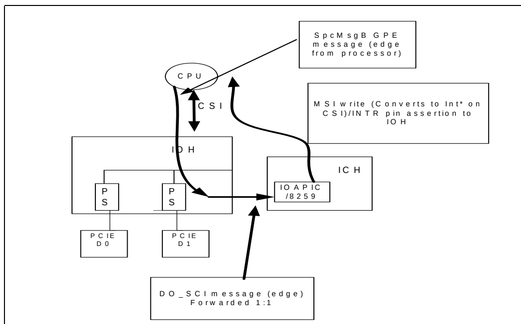
Figure 8-4. Intel® QPI GPE Messages from Processor and DO_SCI Messages from IOH
